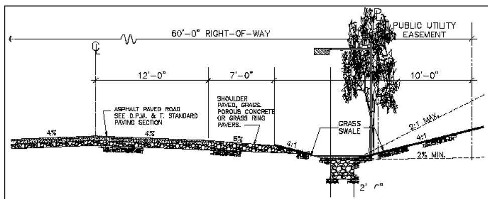
Figure 4.1-1 Alternate Roadway Section without Gutters
